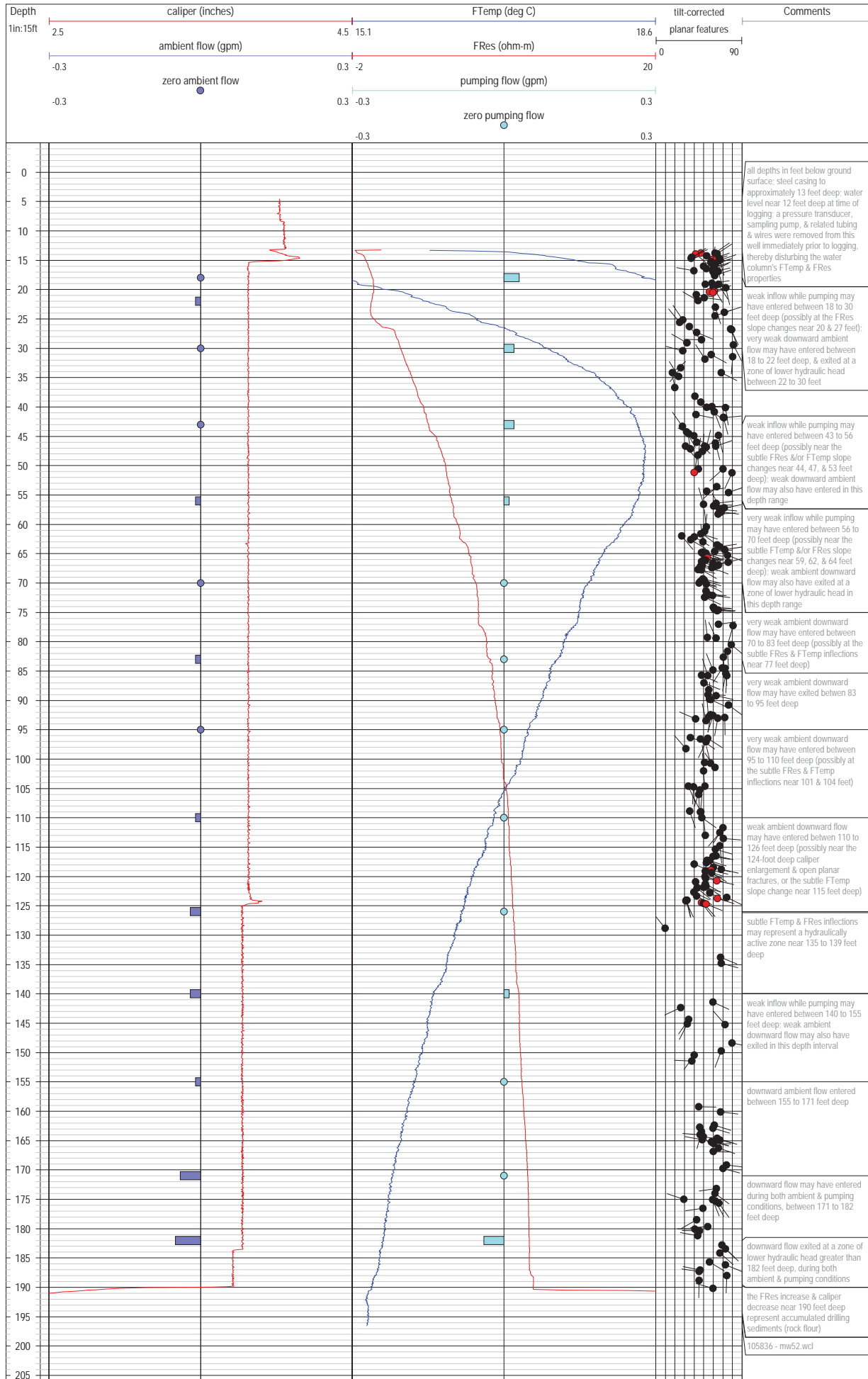
Well: GZA / Buchanan, NY - MW-52 conventional logs
